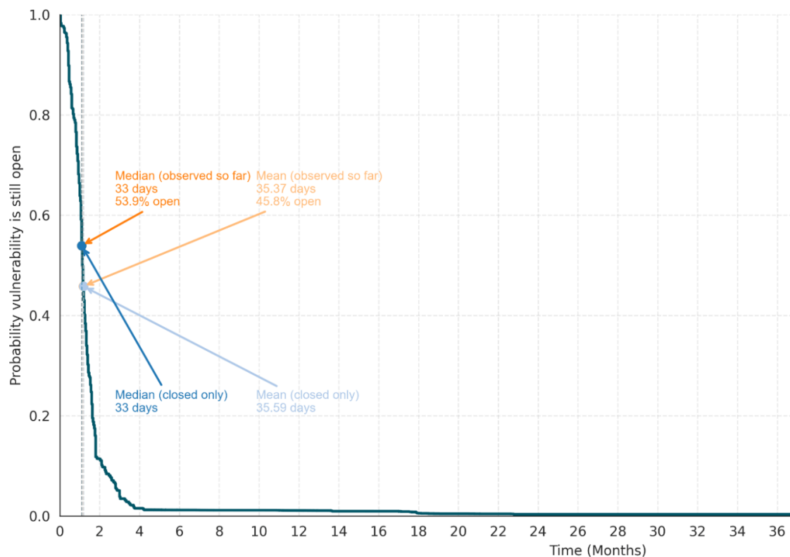
Figure 2: The Kaplan-Meier curve of the time-to-patch of vulnerabilities, versus a probability that a vulnerability is still open, also showing mean and median values. Source: Voicu and Fouque, 2025
