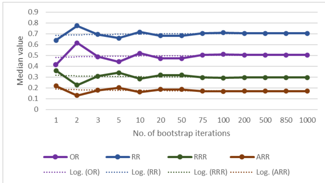
Figure 10: Median values of risk reduction parameters depending on number of bootstrap iterations
