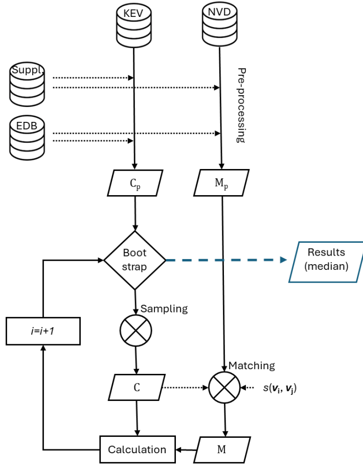
Figure 9: PSIRT efficiency assessment model based on matched case-control methodology with bootstrapping
