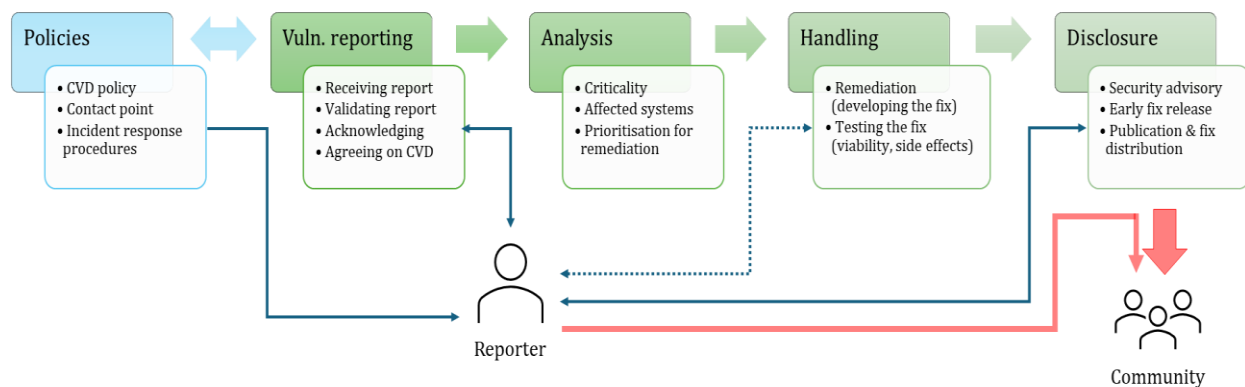
Figure 5. PSIRT role in a CVD process.
