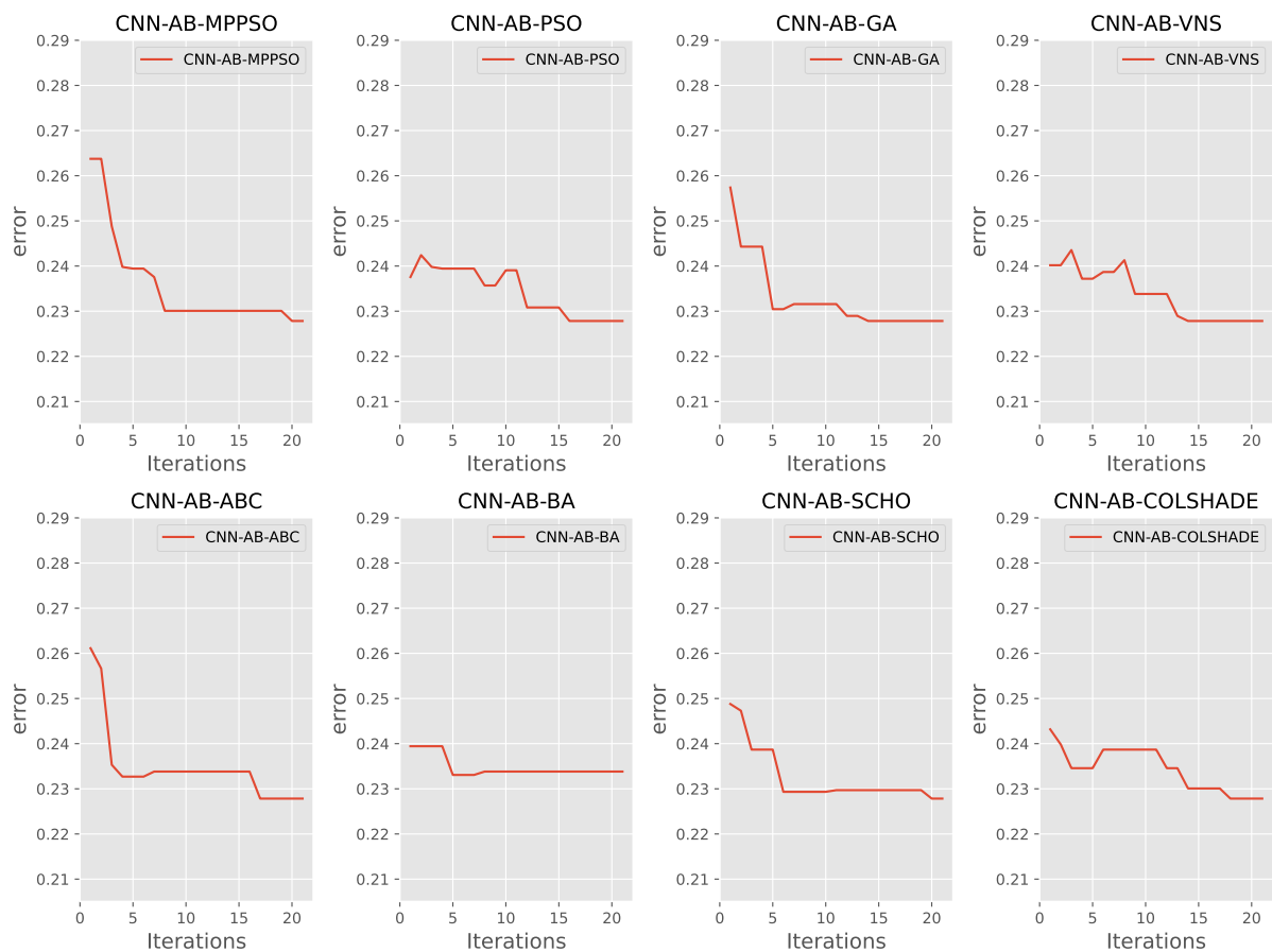
NASA L2 Framework CNN-AB - error convergence graphs
