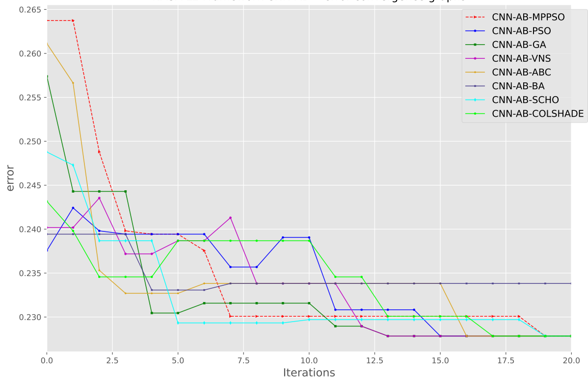
NASA L2 Framework CNN-AB - error convergence graphs
