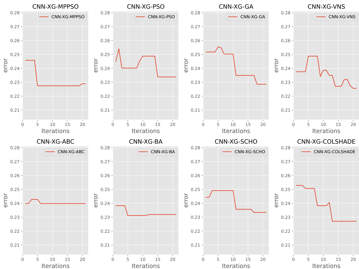
NASA L2 Framework CNN-XG - error convergence graphs
