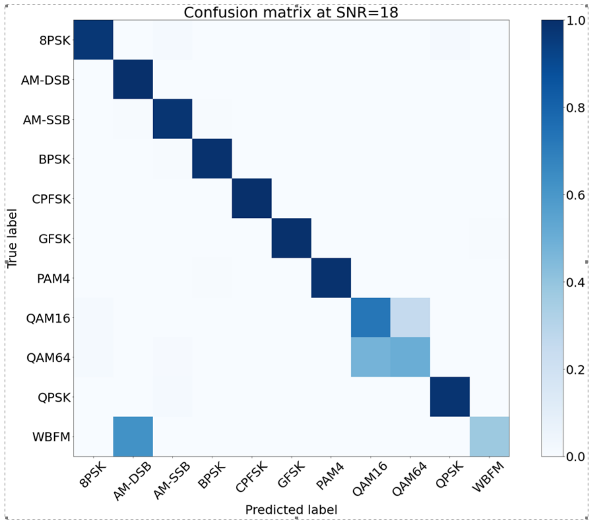
Figure 7-2 Performance of CNN deep LSTM [163]
