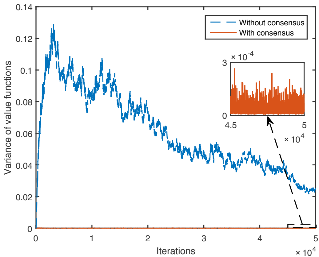
Figure 6-6 Statistics of errors in estimations of state-value function for different algorithms as a function of the number of iterations [43]
