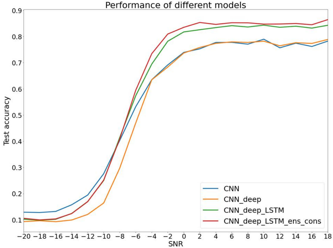
Figure 7-1 Different deep learning models for different SNRs [163]
