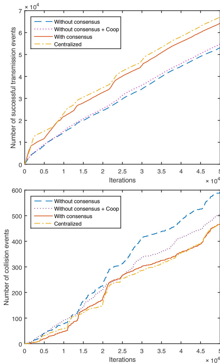
Figure 6-10 Total count of transmission events within the network, both successful and failed, for different algorithms as a function of the number of iterations [43]
