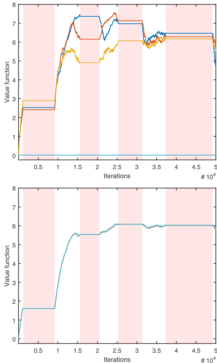
Figure 6-7 Estimations of the value function performed by all agents, both without consensus (upper figure) and with consensus (lower figure), shown with different lines, for a state which can only be visited by three agents. Times while the channel in question is occupied by primary users are shaded in red. [43]
