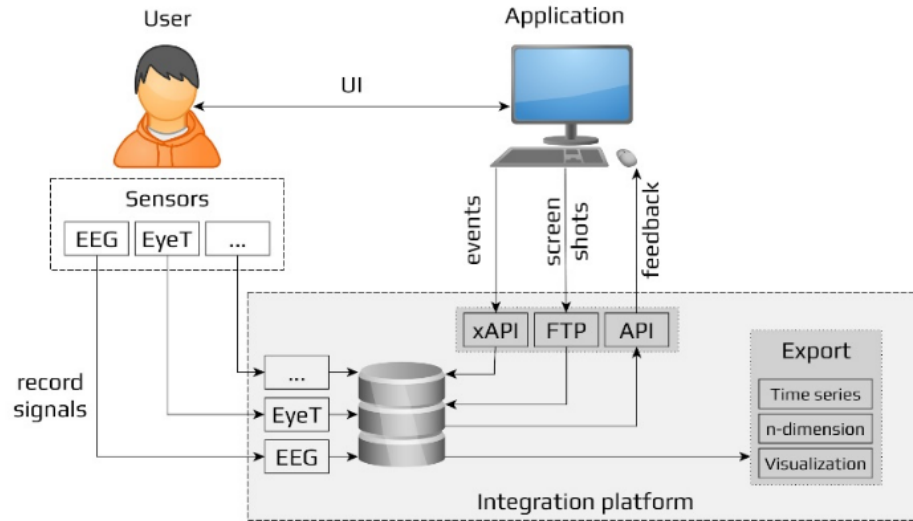
Figure 5.2: HCI monitoring and analytics platform (HCI.MAP), [45].
