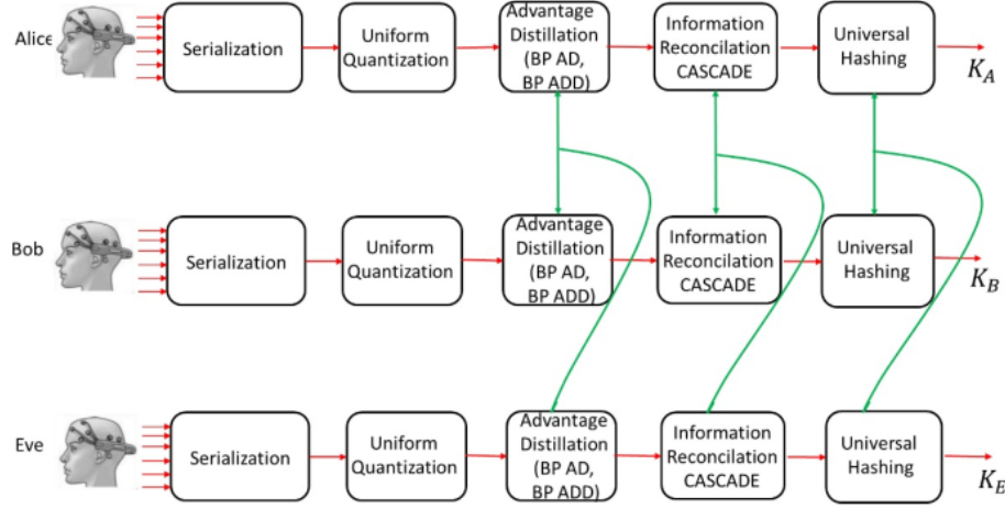
Figure 5.11: The proposed SKD system architecture is designed based on the asynchronous EEG data of the participants. Messages transmitted on the publicly available channel are indicated by the color green.
