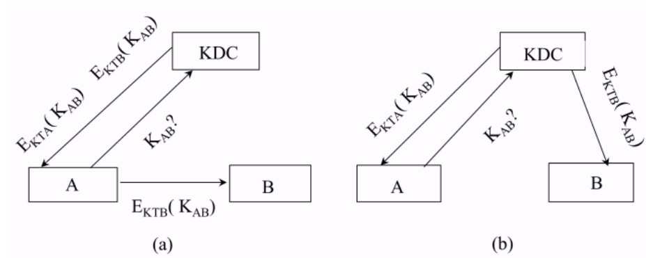
Figure 4.2: Centralized exchange of cryptographic keys
