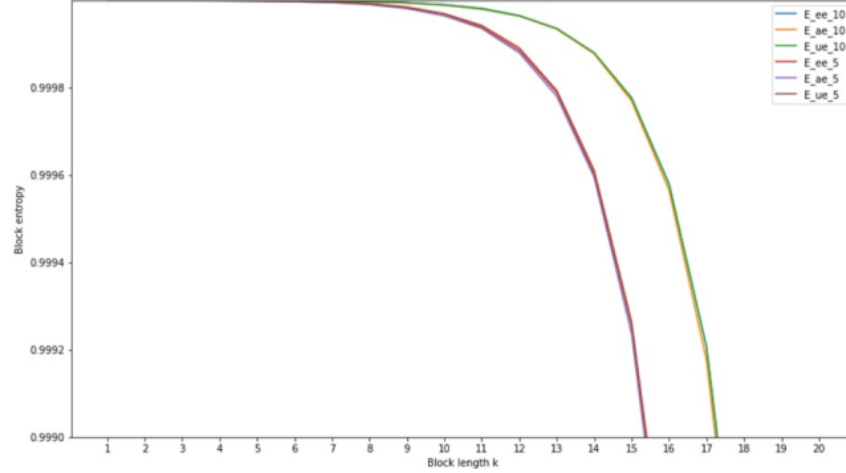
Figure 5.16: Results of the proposed SKD system regarding block entropy for booth quantization possibilities, n_b = 5 and n_b = 10 bits, for all attacker types
