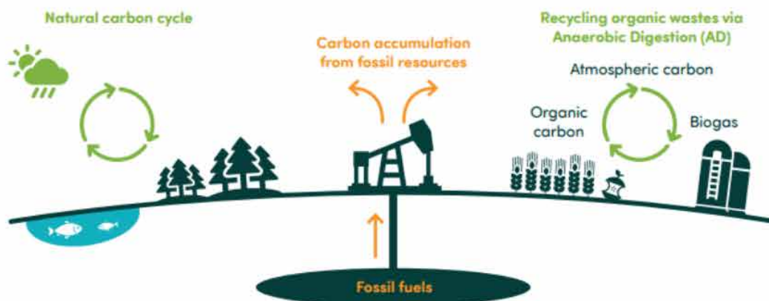
Slika 5. Kruženje ugljenika (izvor: https://www.epa.gov/climate-indicators/climate-change-indicators-global-greenhouse-gas-emissions )
