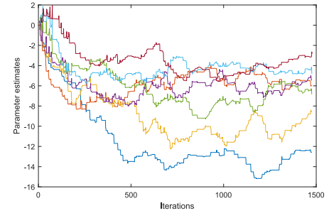
Fig. 6. Parameter estimates obtained in single-agent case using GTD2( \lambda ) algorithm. Each color corresponds to a different parameter (with seven parameters total).
