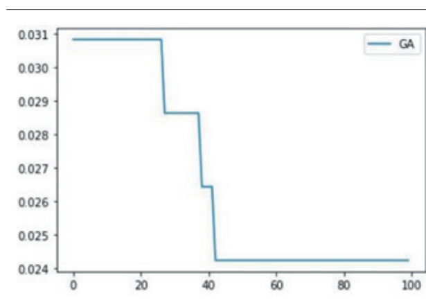
Figure 3. Convergence graph.
