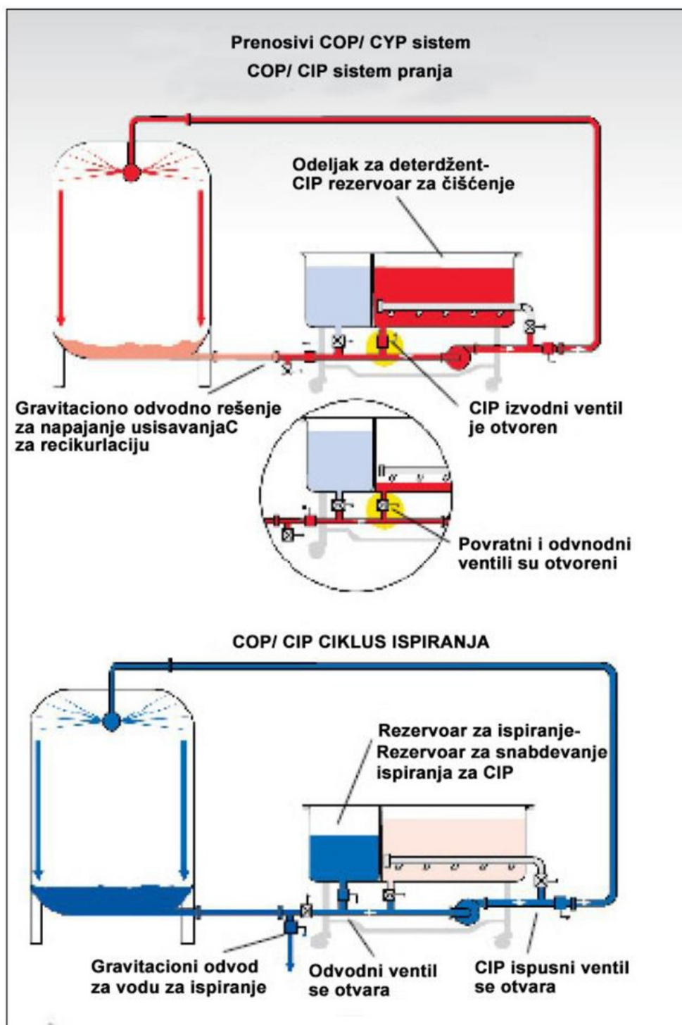
Slika 14: Portabl COP/CIP system
