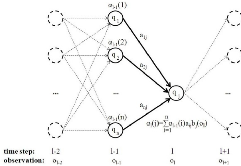
Figure 2.6: The forward trellis.
