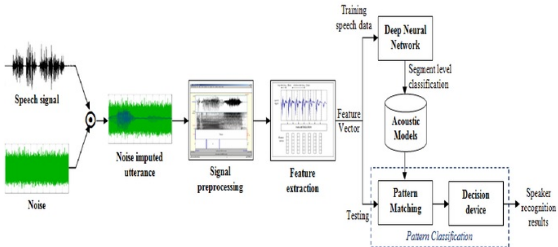
Figure 5.1: Automatic speaker recognition system architecture.
