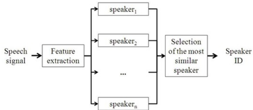
Figure 1.3: Closed-set identification diagram. The resulting speaker ID belongs to one of the speakers available in the database.
