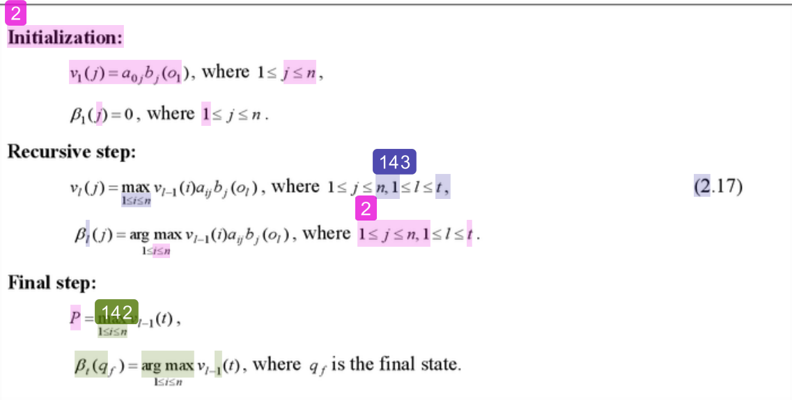
Figure 2.7: The Viterbi algorithm.
