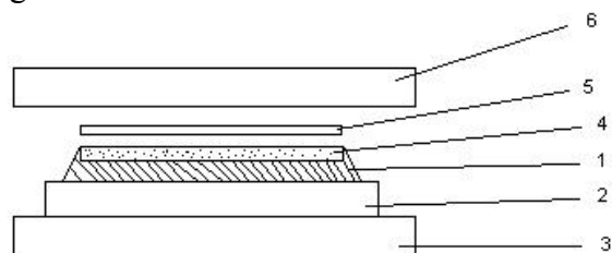
Fig. 7. Realization of the polyurethanes standard mould
