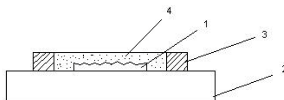
Fig. 4. Obtaining of the silicone mould: 1-experimental primary model; 2-platform of the pressing machine; 3-polyurethanes frame; 4-silicone rubber mould
