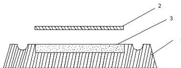
Fig. 2. Mould used for the stamping of the plastically pulp 1-silicone mould with a collecting channel; 2- stamped part; 3-plastisol pulp
