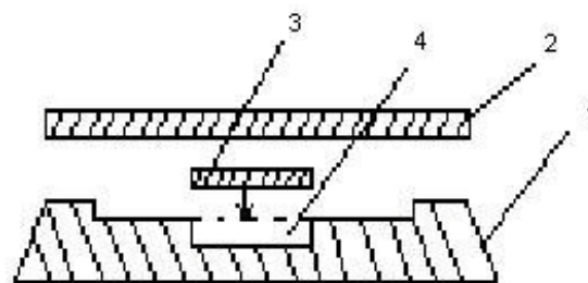
Fig. 1. Mould used for the simultaneously stamping of the two parts 1-silicone mould; 2- part A; 3- part B; 4- cavity for the stamping of the part B
