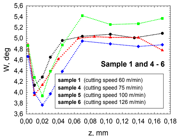
Fig. 12. Average width of the \{211\} diffraction line obtained for samples 1, 4, 5, and 6.
