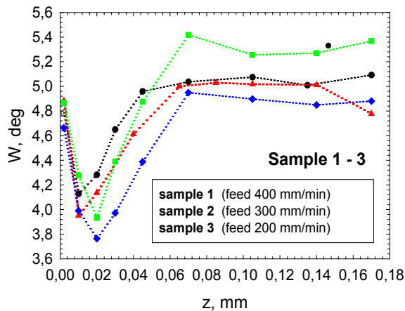
Fig. 11. Average width of the \{211\} diffraction line obtained for samples 1, 2, and 3.
