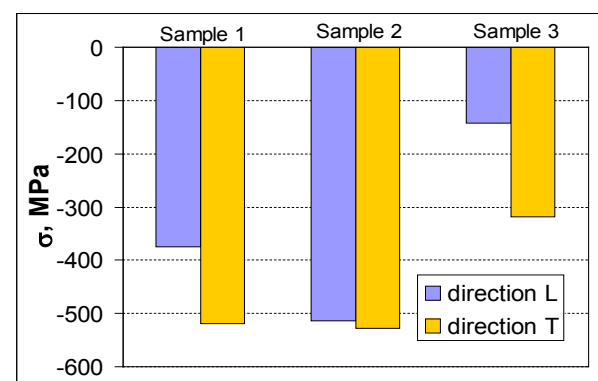
Fig. 3. Average values from areas P1 and P2 of residual stresses \sigma_L and \sigma_T , MPa from the surface;
