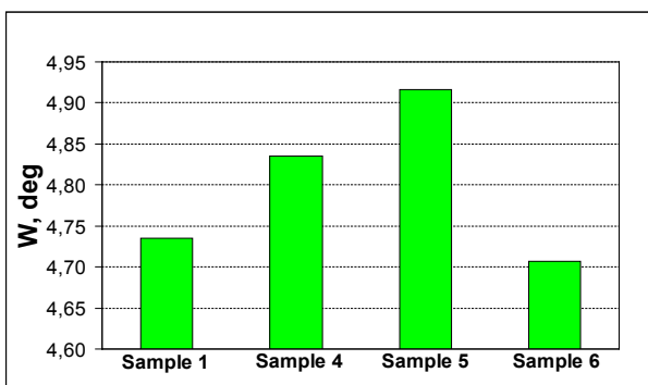
Fig. 6. Average values of the width of the \{211\} diffraction line obtained from areas P1 and P2 from the surface; relation of residual stresses on the cutting speed modification.
