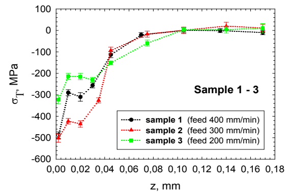
Fig. 8. Depth distribution of residual stresses \sigma_T obtained for samples 1, 2, and 3.
