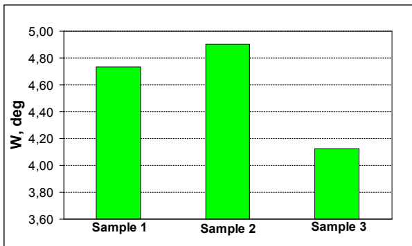
Fig. 5. Average values of the width of the \{211\} diffraction line obtained from areas P1 and P2 from the surface; relation of residual stresses on the feed modification.
