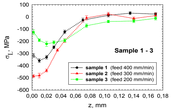
Fig. 7. Depth distribution of residual stresses \sigma_L obtained for samples 1, 2, and 3.
