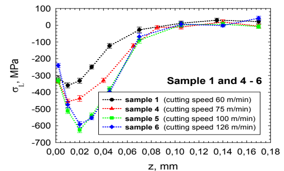
Fig. 9. Depth distribution of residual stresses \sigma_L obtained for samples 1, 4, 5, and 6.
