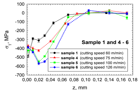
Fig. 10. Depth distribution of residual stresses \sigma_T obtained for samples 1, 4, 5, and 6.
